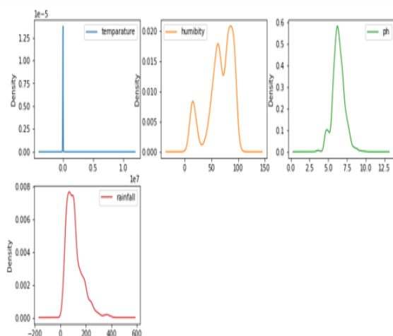
Fig 5: Density Diagram
