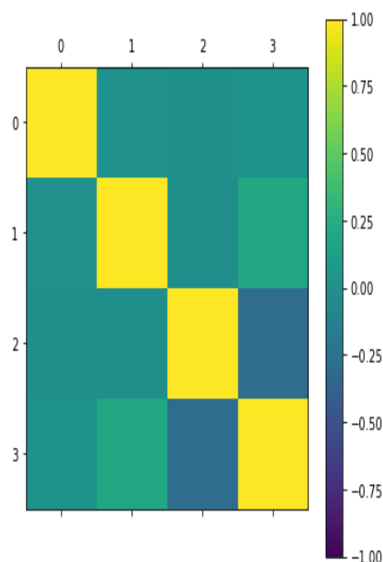
Fig 7: Correlation diagram
