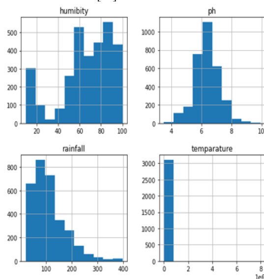
Fig 4: Hist Diagram
