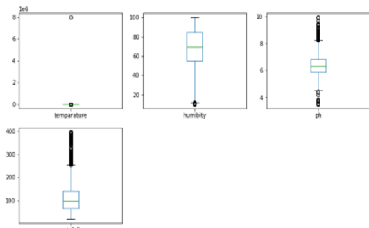
Fig 6: Box Diagram
