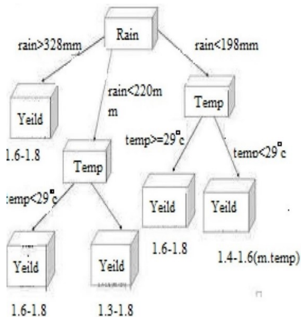
Fig 2: Decision tree
